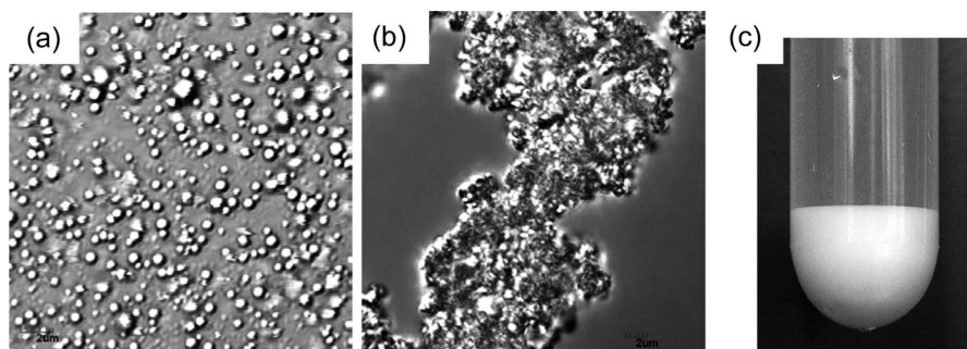
Figure 1. Laser scanning confocal microscopy images of (a) freshly prepared hybrid catalyst 1d–2a in water and (b) catalyst 1d–2a in water after its sixth reuse. Picture (c) refers to fresh 1d–2a in water.
